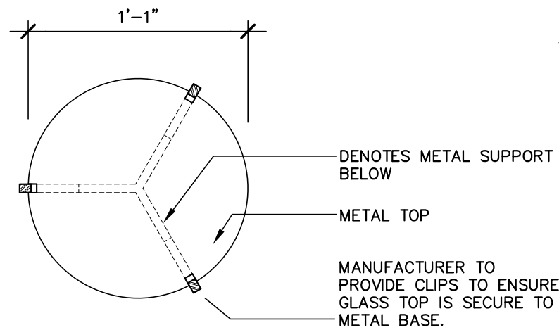
1B PLAN DETAIL SCALE: 1 1/2" = 1'-0"
