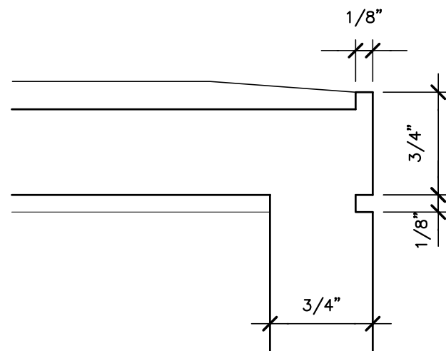
2B SECTION DETAIL SCALE: FULL SCALE
