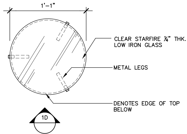
1A PLAN DETAIL SCALE: 1 1/2" = 1'-0"
