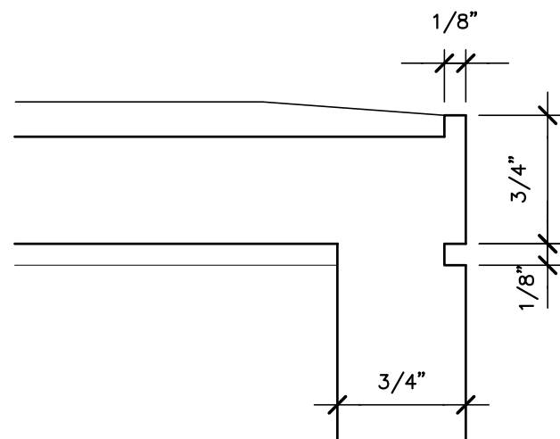
2B SECTION DETAIL SCALE: FULL SCALE
