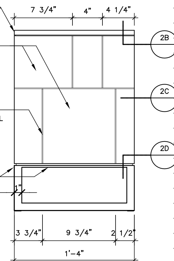
1C SIDE ELEVATION SCALE: 1 1/2"=1'-0"
