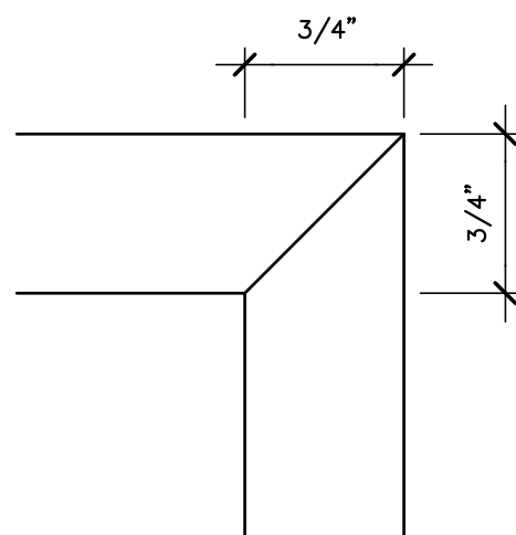
2C PLAN DETAIL SCALE: FULL SCALE
