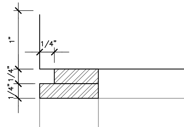
2D LEG SECTION DETAIL SCALE: FULL SCALE
