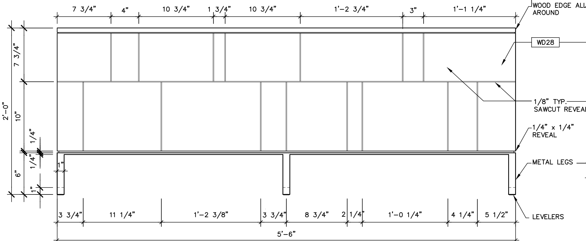
1B FRONT ELEVATION SCALE: 1 1/2"=1'-0"
