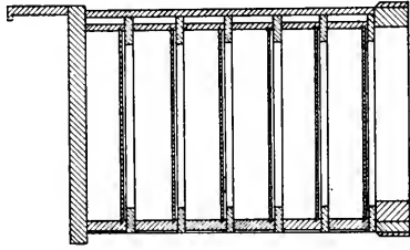
SECTION ON LINE A-A
