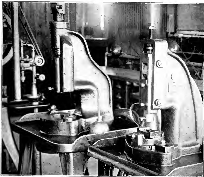
Screw Press
